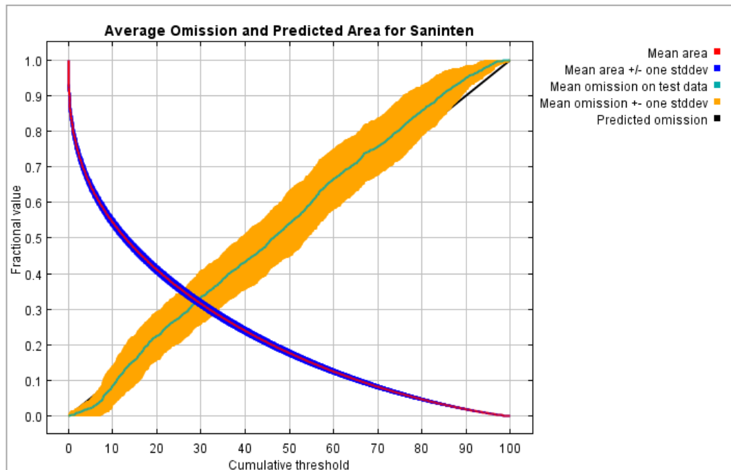
Gambar 50. Kurva average omission and predicted area
