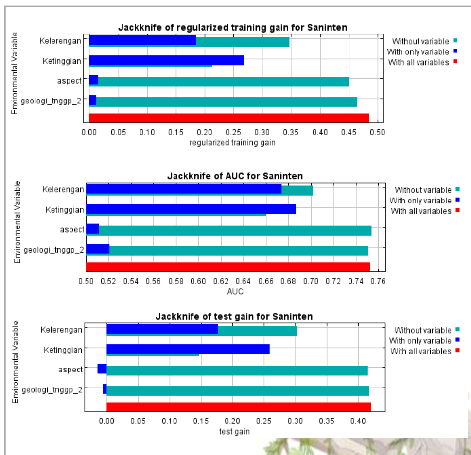
Gambar 58. Hasil Uji Jackknife
