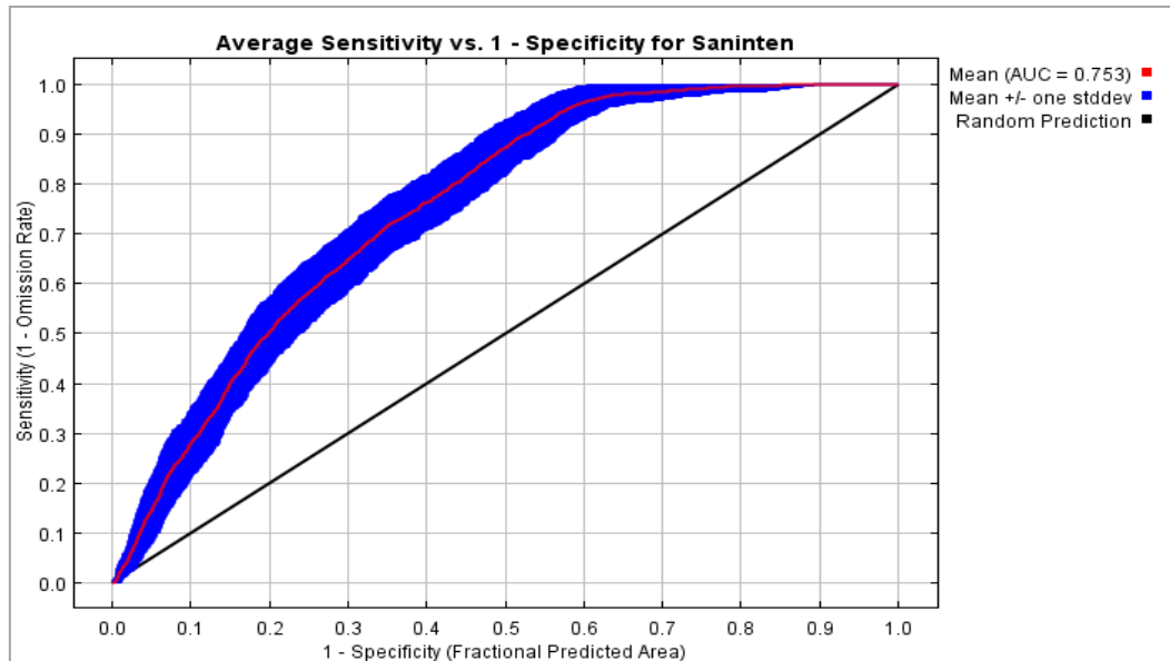
Gambar 51. Kurva sensitivity and specificity
